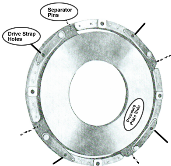
Intermediate Plate Part No. 125197
