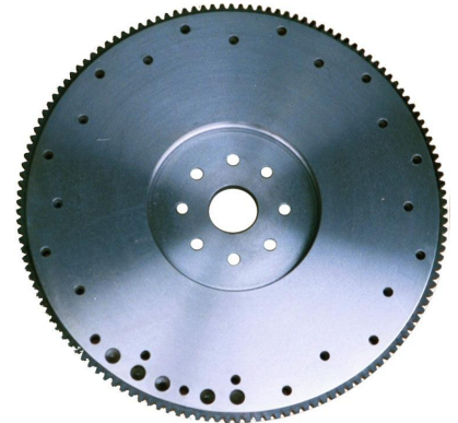
DETROIT FWN8922126 Style: FLAT Application: 8.2L Clutch: 13+or 14+ . 8 spring disc Bearing: #205 7.125+bore, 8 mounting holes 17+ring gear with 138 teeth List Price $470.84
